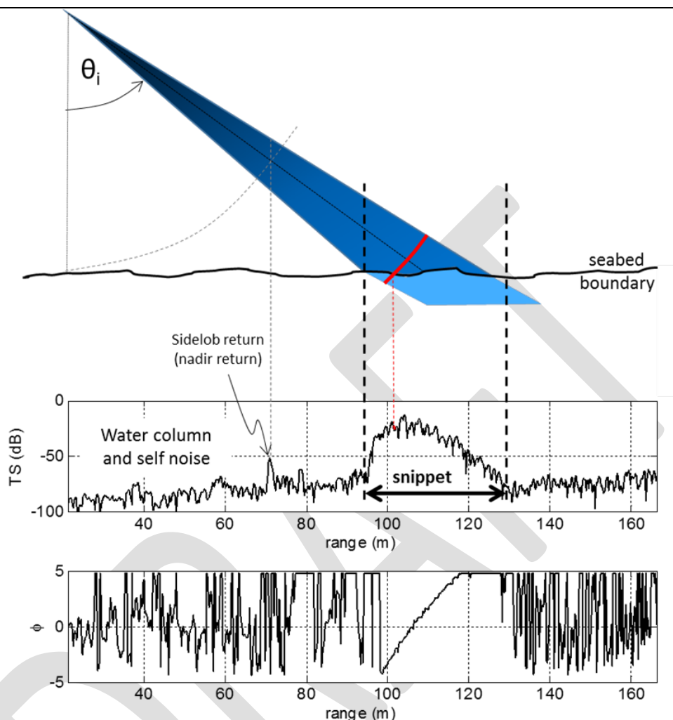
Figure 2-14 An example of the interaction of a pulse at oblique incidence and the generation of a snippet.
