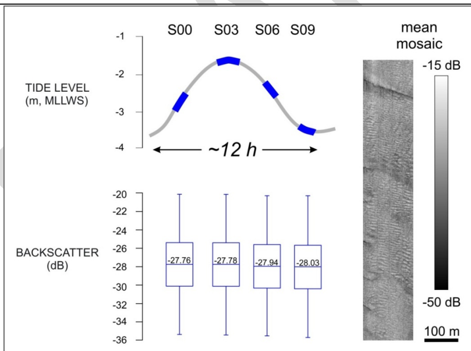
Figure 3-5 Evaluation of Backscatter Strength (BS) variance from successive measurements during a tide cycle ( \sim 12 h); 4 surveys of the same area with constant input and runtime parameters; boxplots of the BS data with mean values; for the four data sets, the statistics are calculated from each mosaics values (resolution = 1 \times 1 m) on the common rectangular area presented in the figure; very low dispersion of the 4 mean values: standard deviation = 0.1 dB; data from Kongsberg EM1002 MBES on RV Belgica.
