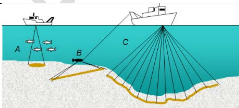
Figure 1-2 Schematic representation of the three main types of seafloor-mapping sonars (A: single-beam echosounder; B:
