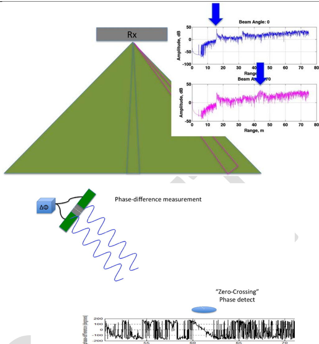
Figure 4-7 Illustrations above provide examples of amplitude (a) and differential phase zero-crossing detections (b). Beam amplitude time series are shown for near-nadir beams (blue) and oblique beams (magenta). The bottom produces a sharp peak in the former from which an accurate detection is possible in the near-nadir beams and a broad peak from which an accurate detection is not possible in the oblique beams. For this reason amplitude detects alone are used for near-nadir beams. For oblique beams, the steered receive array is split into sub-apertures from which the differential phase of the received signal is measured. When the pulse passes the intersection of the beam and the seafloor a characteristic phase-ramp is produced in the differential phase time series. The zero-crossing of this phase ramp is used to mark the two-way travel time of the pulse along this beam.
