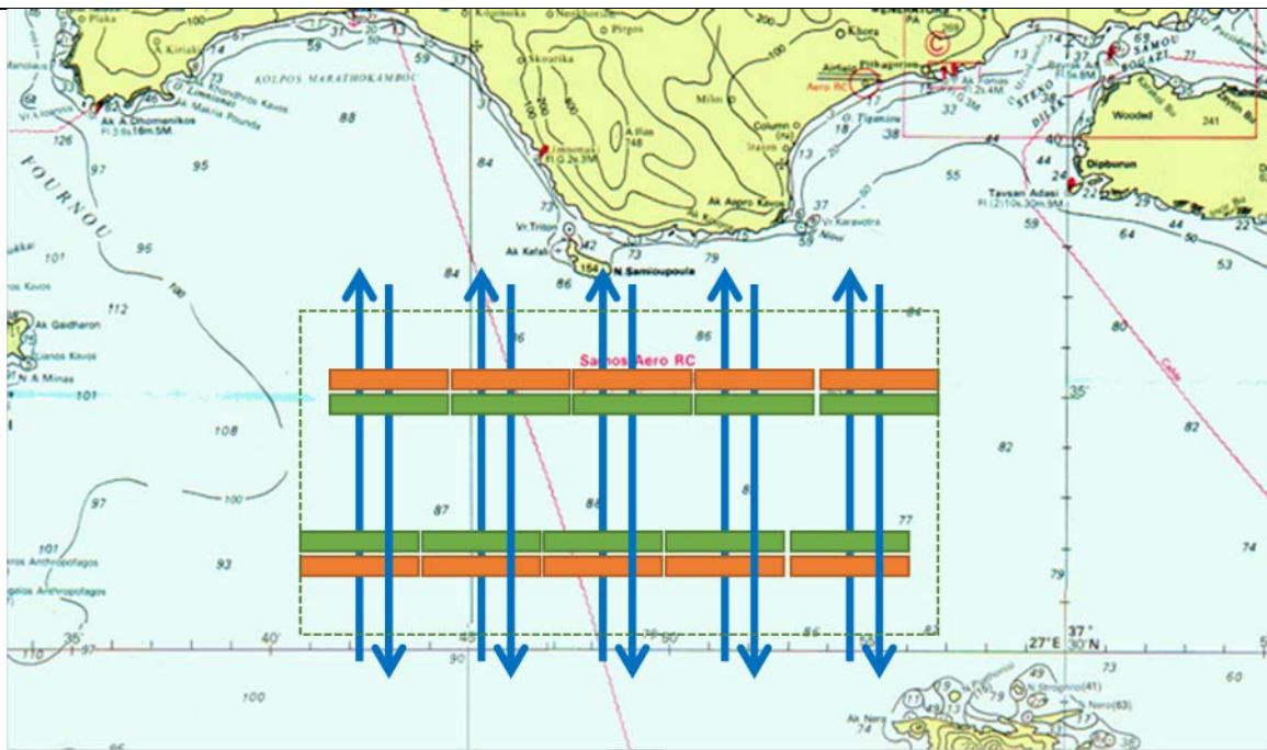
Figure 5-15 For phase measuring systems, green area with full bathymetry coverage. The nadir of every line is also covered by the adjacent line, which improved the data density of that area as well as it allows sensing the angular backscatter response of the seafloor at two different angles.
