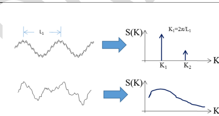
Figure 2-9 Spatial spectrum of a rough surface. The power spectrum, as a function of the spatial wavenumber, may be composed either of discrete lines (is the relief is a summation of a few sine contributions – see upper plot) or a continuum of components in case of a random relief (see lower plot).
