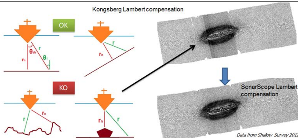
Figure 6-5 Example of artefact induced by sonar hardware gains and compensated in post-processing. Here, the dynamic gain implemented in a Kongsberg system fails to account for the complex bathymetry induced by a shipwreck lying on a flat seafloor. The removal of this gain followed by a more appropriate compensation of ensonified area in post-processing allows correcting the artefact (Augustin, 2013, data courtesy of Shallow Survey 2012, processed with SonarScope).
