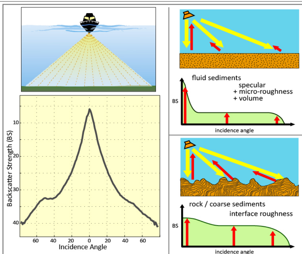
Figure 1-4 The angular dependence of Backscatter Strength (BS). The rapid decrease in the BS intensity with incidence angles shows well in the BS angular profile (bottom left): high BS values at the nadir ( 0^\circ incidence) decrease rapidly with gazing angle. The shape of the angular profile is directly influenced by the interface roughness (right); it is not necessarily symmetrical in practice (example shown here), depending on local features
