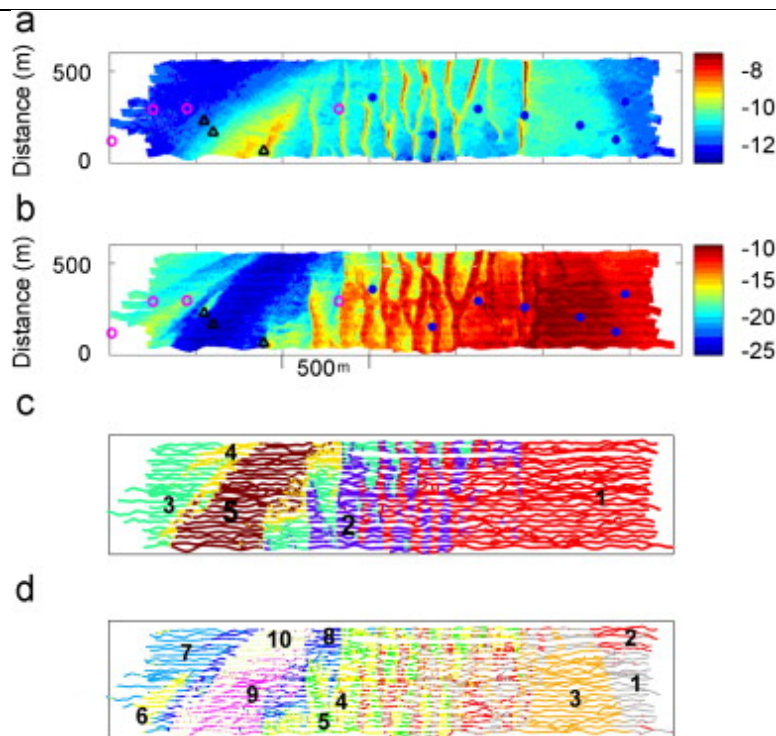
Figure 3-16 Results of mapping of Keppel Bay multibeam data (from Hamilton and Parnum, 2011). (a) bathymetry with sediment sample locations. Symbols: Dark blue circles are coarse sand and shell debris, mauve rings are muddy sand, and triangles are mud or sandy mud, (b) mean Backscatter Strength (dB) averaged over 40–60. (c) mapping of five acoustic classes from a direct clustering of BS curves and (d) mapping of 10 acoustic classes from a direct clustering of BS curves.
