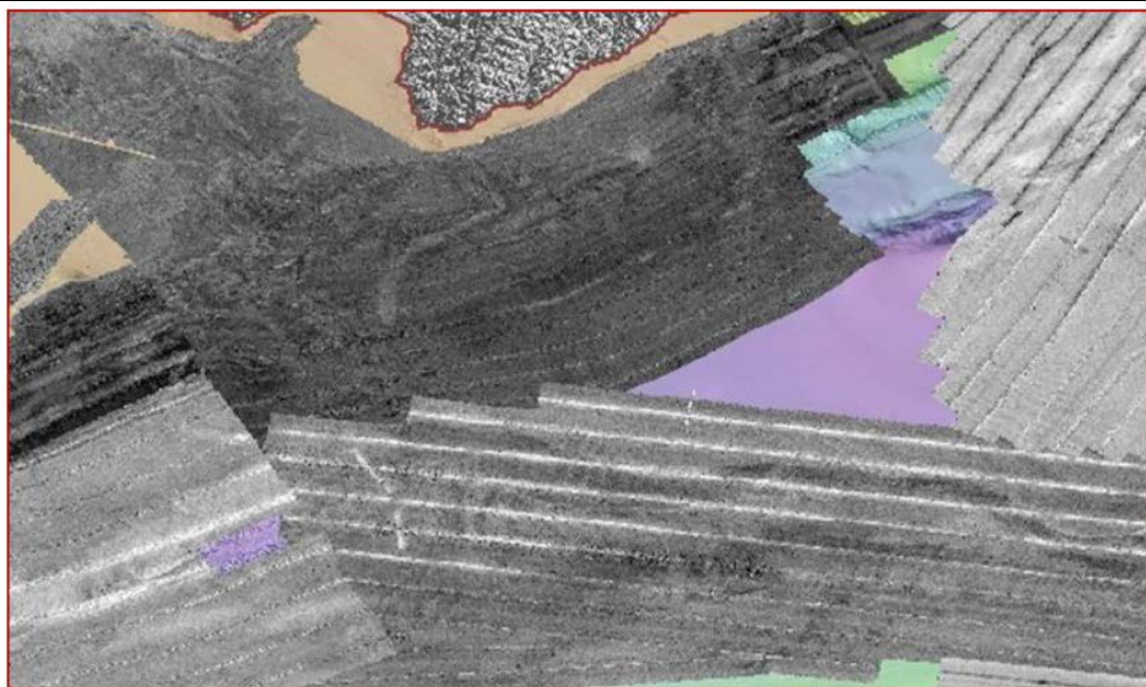
Figure 1-1 Example of multiple backscatter surveys collected in the same area during different survey cruises using the same MBES (Cook Straits, NZ; the sonar was the EM 300 on R/V Tangaroa). This figure illustrates the discrepancy between the reflectivity by one same MBES along the years. Regardless of the equipment used and the post-processing sequence applied, the overlapping regions should produce a similar image, which is obviously not the case here.
