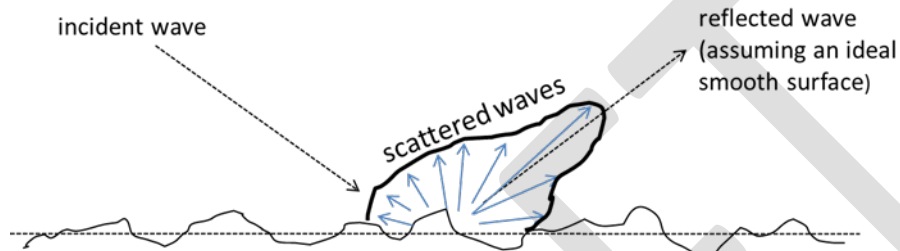
Figure 2-6 The reflected and scattered waves arising from the incidence of an acoustic wave upon a rough surface.
