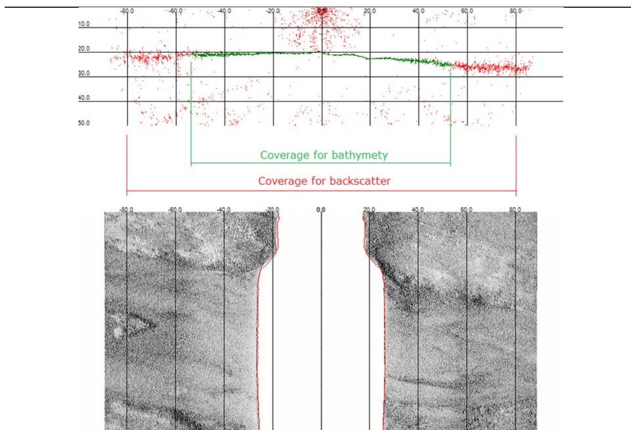
Figure 5-14 Data example from a PMBS, illustrating the difference between effective swath width for bathymetry (green) and backscatter (red).
